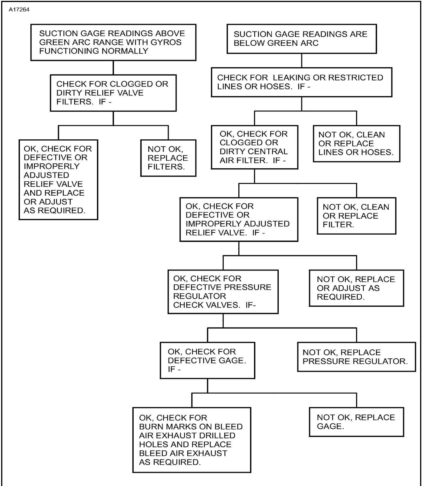
Figure 101 : Sheet 1 : Vacuum System Troubleshooting
