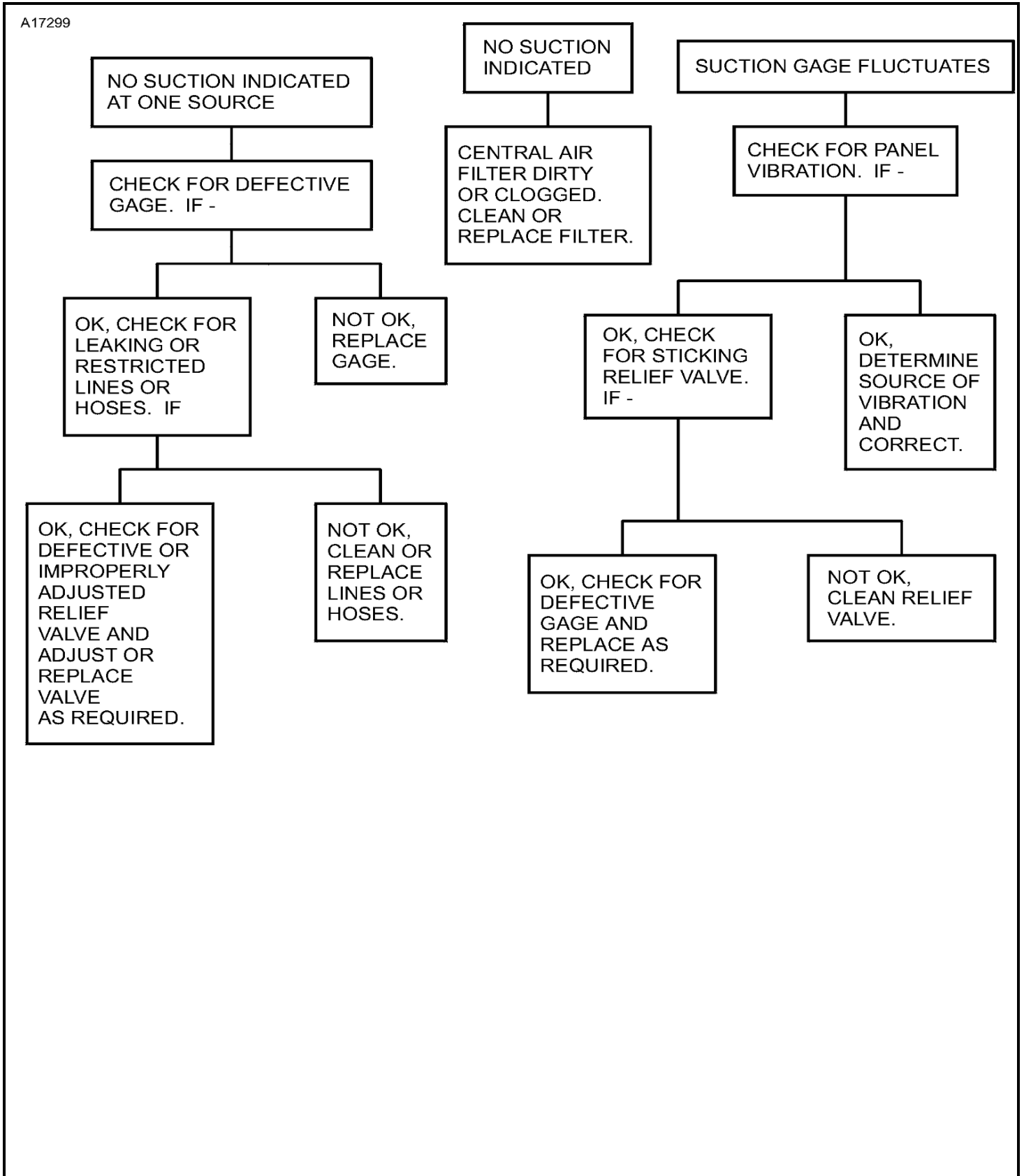
Figure 101 : Sheet 2 : Vacuum System Troubleshooting
